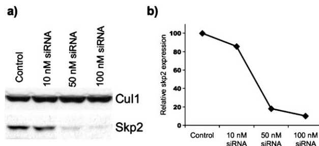
Fig. 2 Lipitoid transfects siRNA and causes concentration dependent downregulation of the targeted protein. Varying concentrations (10 nM–100 nM) of skp2 siRNA2 were tested in T98G cells. Transfection experiments were done with the lipitoid DMPE-(NaeNmpeNmpe) 3 as transfection agent and LacZ siRNA as the control siRNA (50 nM). (a) Western Blot analysis with specific antibodies against skp2 and the loading control cull1 was performed 48 h after transfection. (b) Skp2 amounts as quantified from the Western Blot.
