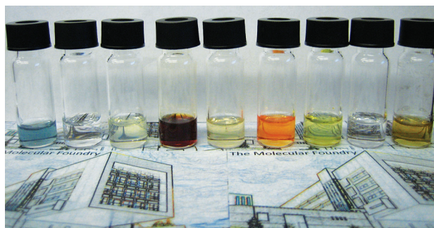
Figure 5. Dispersions of \text{BF}_4^- /DMF passivated nanocrystals. From left to right: ITO, AZO, \text{TiO}_2 , \alpha\text{-Fe}_2\text{O}_3 , CdSe/ZnS ( \lambda_{\text{em}} = 545 \text{ nm} ), CdSe/ZnS ( \lambda_{\text{em}} = 605 \text{ nm} ), CdSe/CdS quantum dot/quantum rods ( \lambda_{\text{em}} = 619 \text{ nm} ), upconverting \text{NaYF}_4:\text{Yb/Tm} , and Ag nanocrystals.
